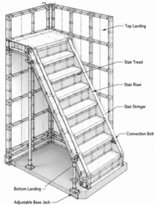
ALUMINUM FORMWORK STAIR SYSTEM DETAIL DRAWING
